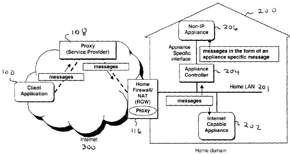
Figure 4: Network Architecture: Communication via (Service Provider) Proxy
