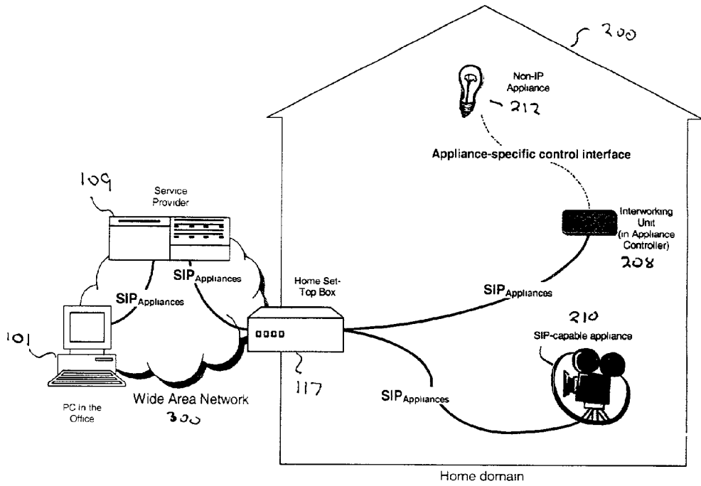
Figure 6. One Possible Physical Realization of Functional Architecture
