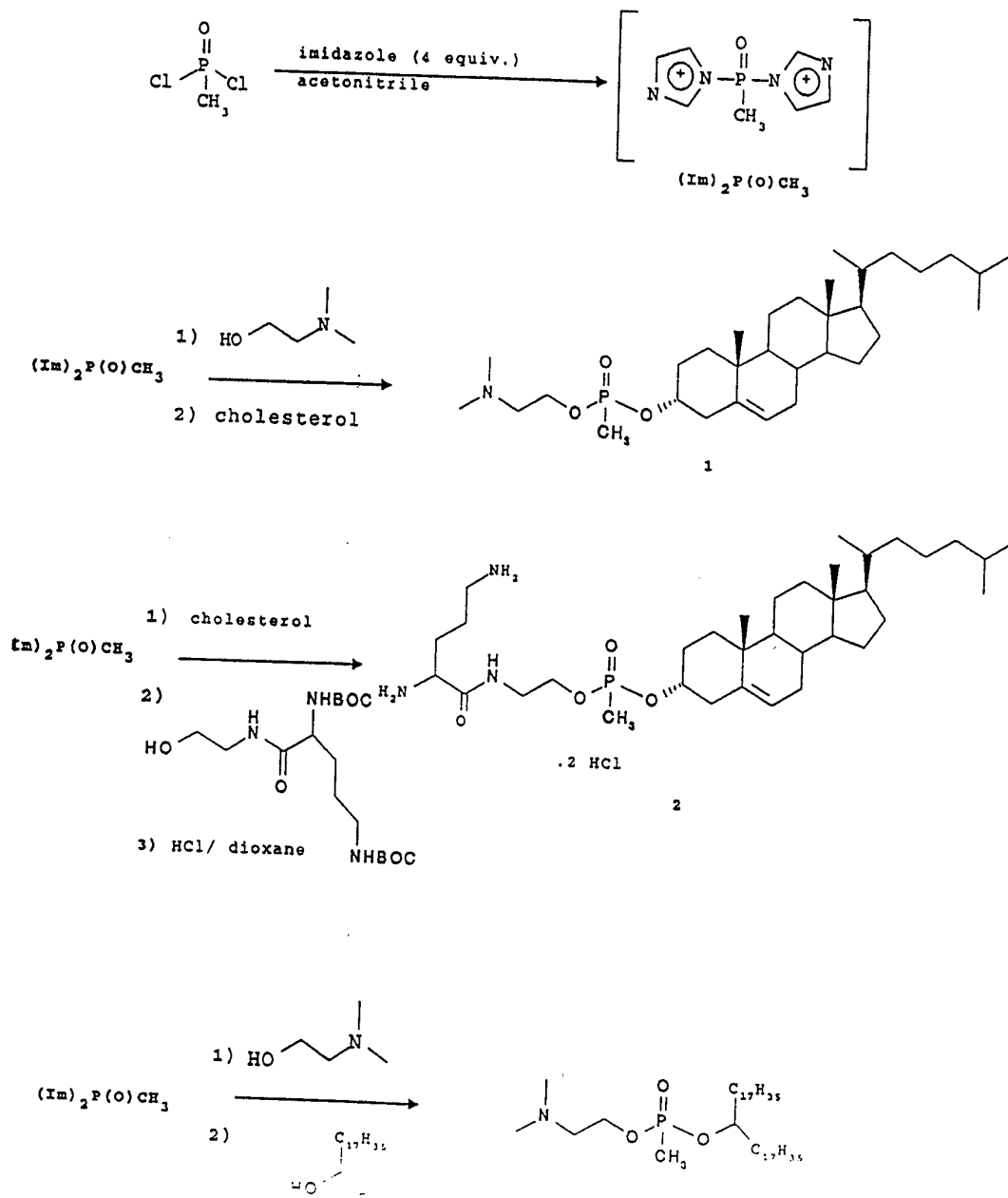
Figure 1: Synthetic scheme for the synthesis of compounds 1, 2 and 3
