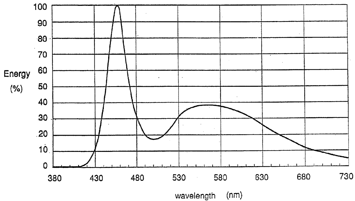
Emission spectrum
