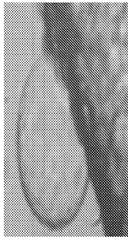
Large Unilamellar QuSome
