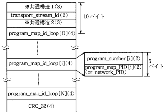
PAT (Program Association Table)
