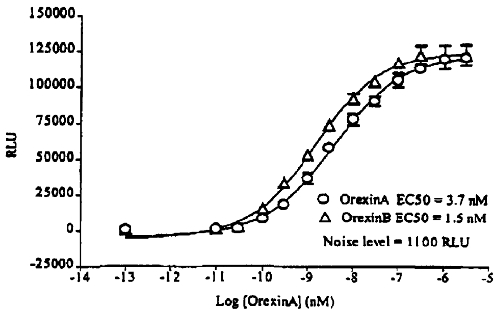
Dose response curve Mix Aequorin-Orexin 2 R
