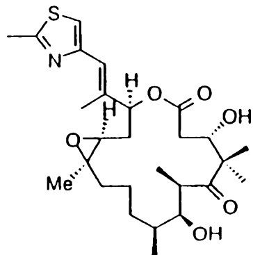
synthetic epothilone B
