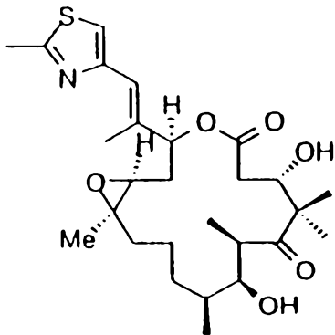
natural epothilone B
