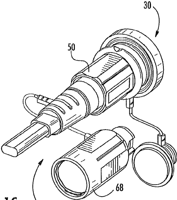
FIG. 1C (PRIOR ART)
