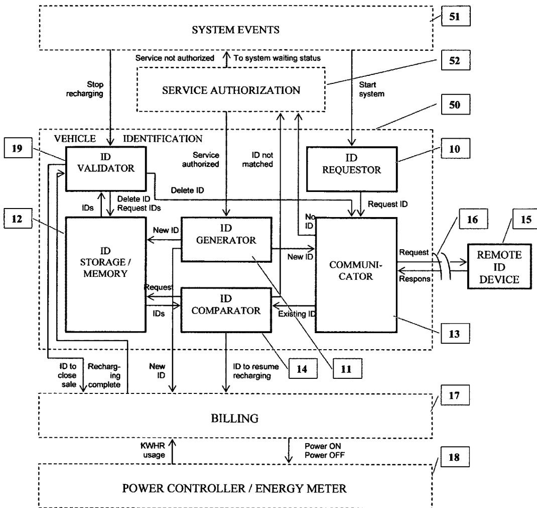
FIG. 2 Vehicle Identification System Functional Diagram
