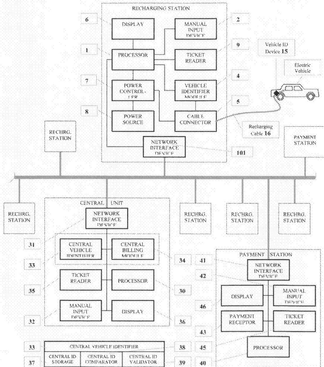
Fig.4 Network of Recharging Stations Block Diagram
