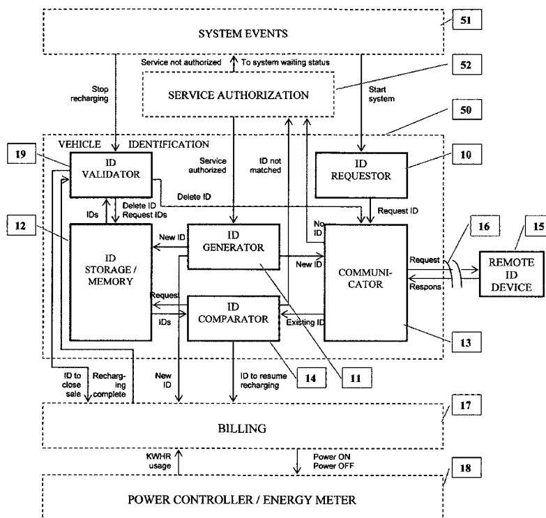
Vehicle Identification System Functional Diagram
