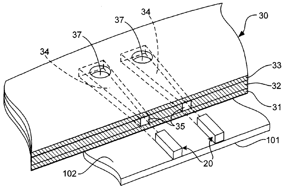
FIG. 11 (PRIOR ART)
