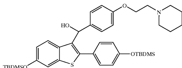
Preparation 1
