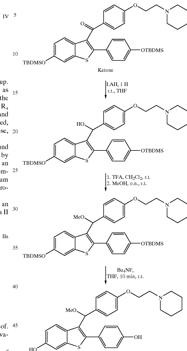
Scheme 1
