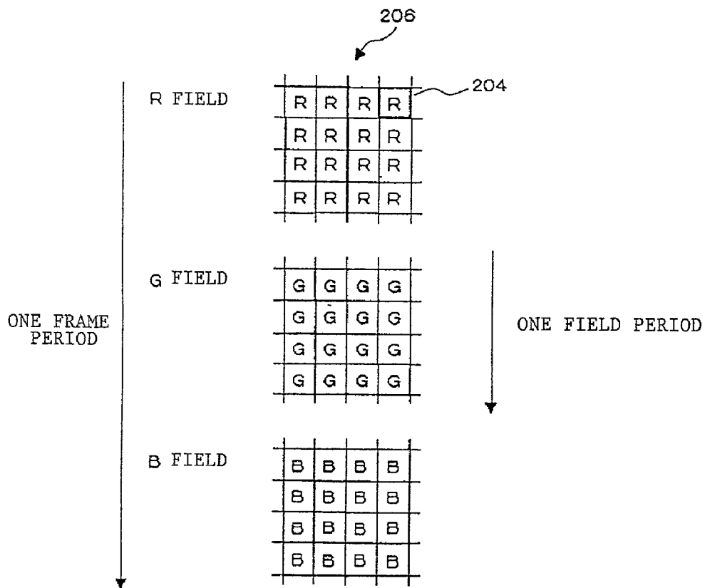
Fig. 2 (Prior Art)
