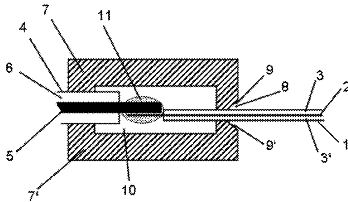
Prior Art
