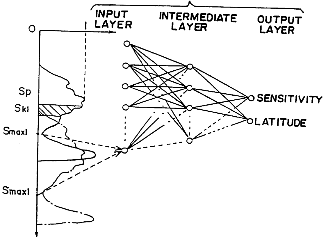
NEURAL NETWORK
