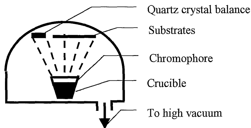
Scheme 3. Diagram of a diffusion vacuum deposition apparatus.
