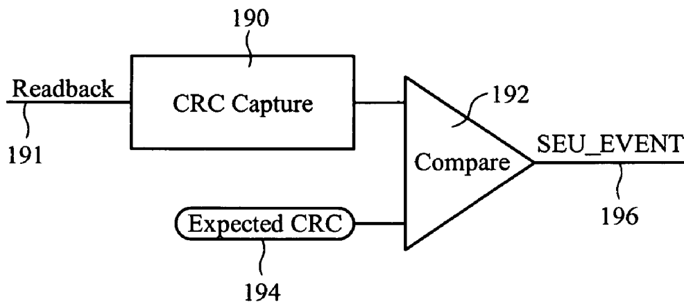
Readback CRCComparator
