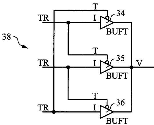
Voting circuit with BUFTs
