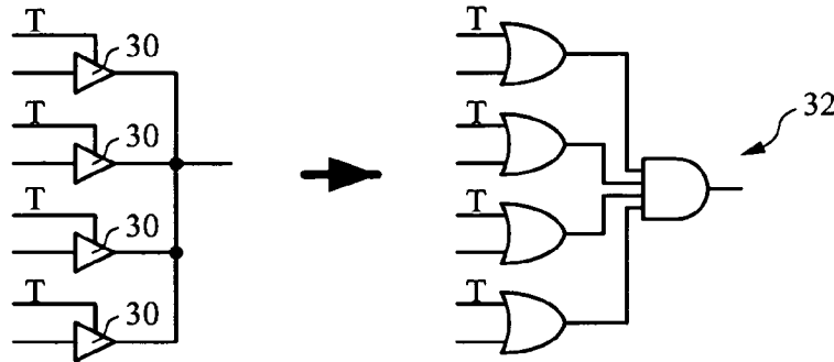
Virtex BUFT Structure
