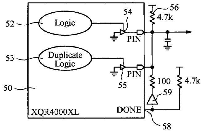
Wire-ANDing Critical Outputs
