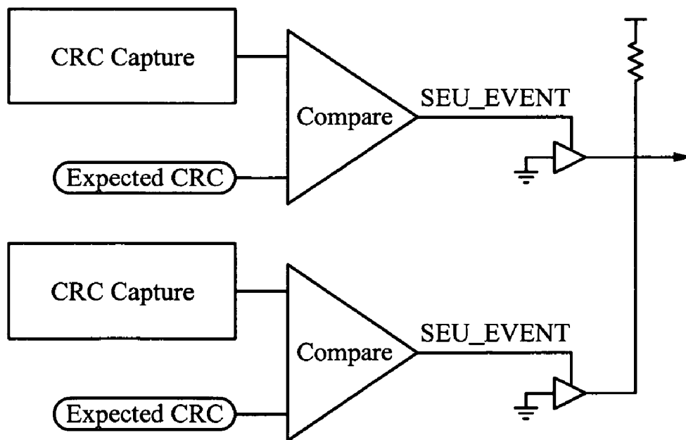
Redundant CRC Comparator
