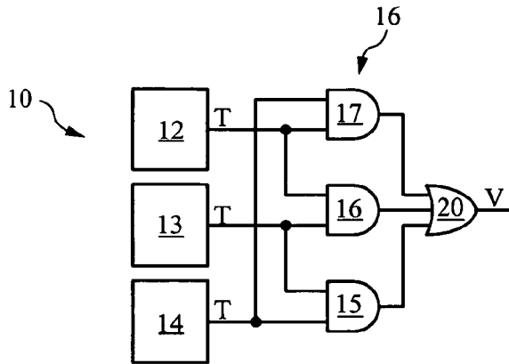
Triple Redundancy with Voting
