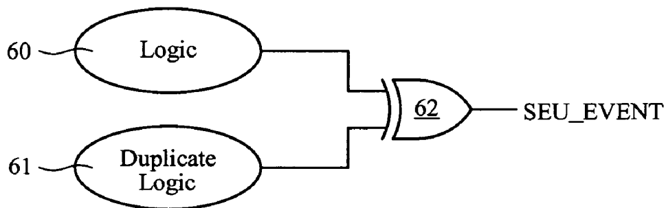
SEU Detection by Reundancy and XOR Gating
