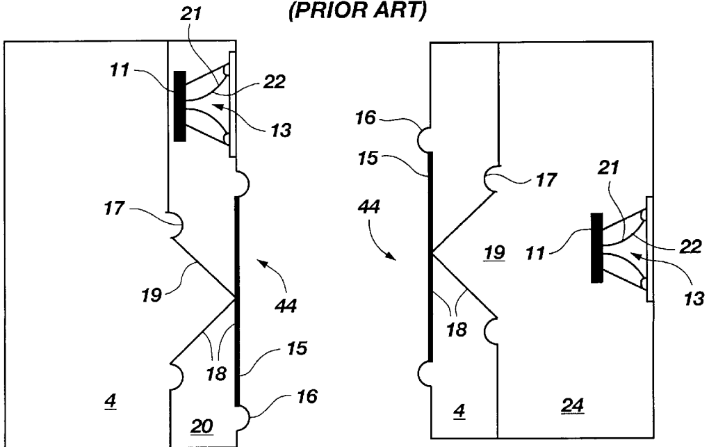
Fig. 3 (PRIOR ART)
