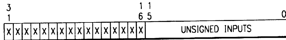
FIG. 10b ("01" IF HEX "8000" X HEX "8000")
