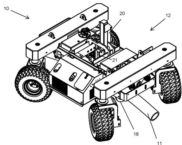
FIG. 1 FOUR WHEEL STEERING
