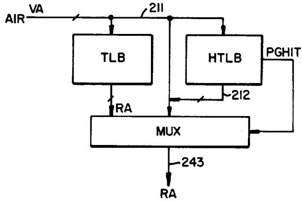
TLB SUBSYSTEM
