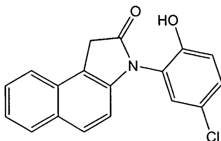
(±)-3-(5-Chloro-2-hydroxyphenyl)-1,3-dihydro-2H-benz[e]indol-2-one.
