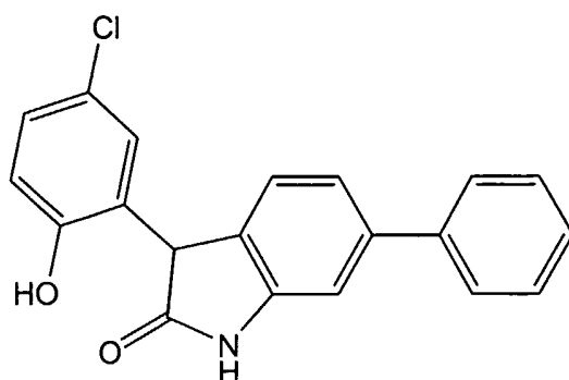
(+)-3-(5-Chloro-2-hydroxyphenyl)-1,3-dihydro-6-phenyl-2H-indol-2-one; and
