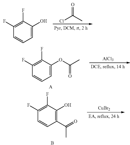
Scheme 1. Synthesis of ARB-1 moiety
