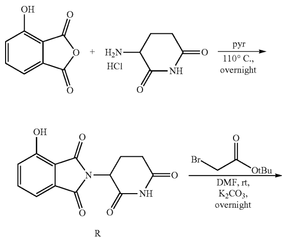
Scheme 4. Synthesis of thalidomide-based E3LB-2 moiety and linker connection
