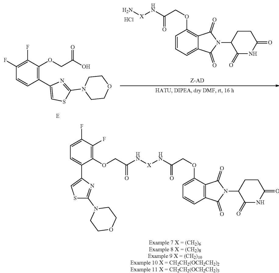
Scheme 5. Synthesis of Examples 7-11
