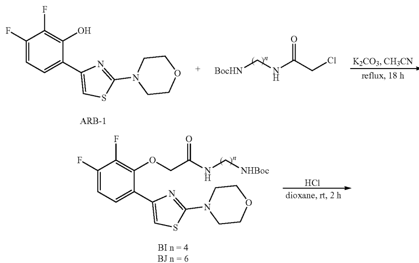
Scheme 11. Synthesis of Examples 22 and 23
