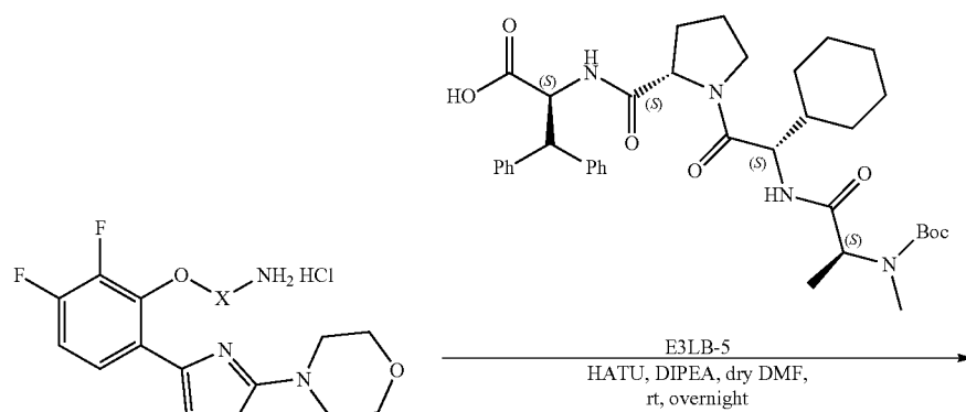
Scheme 13. Synthesis of Examples 24-26
