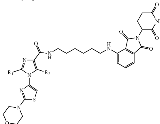
Example 32 R 1 = R 2 = H Example 33 R 1 = R 2 = Br
