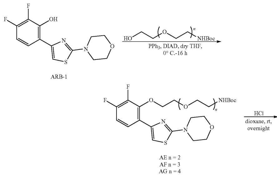
Scheme 6. Synthesis of Examples 12-14
