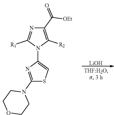
ARB-3 R 1 = R 2 = H ARN-4 R 1 = R 2 = Br
