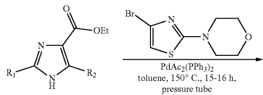
Scheme 18. Synthesis of Examples 32-33
