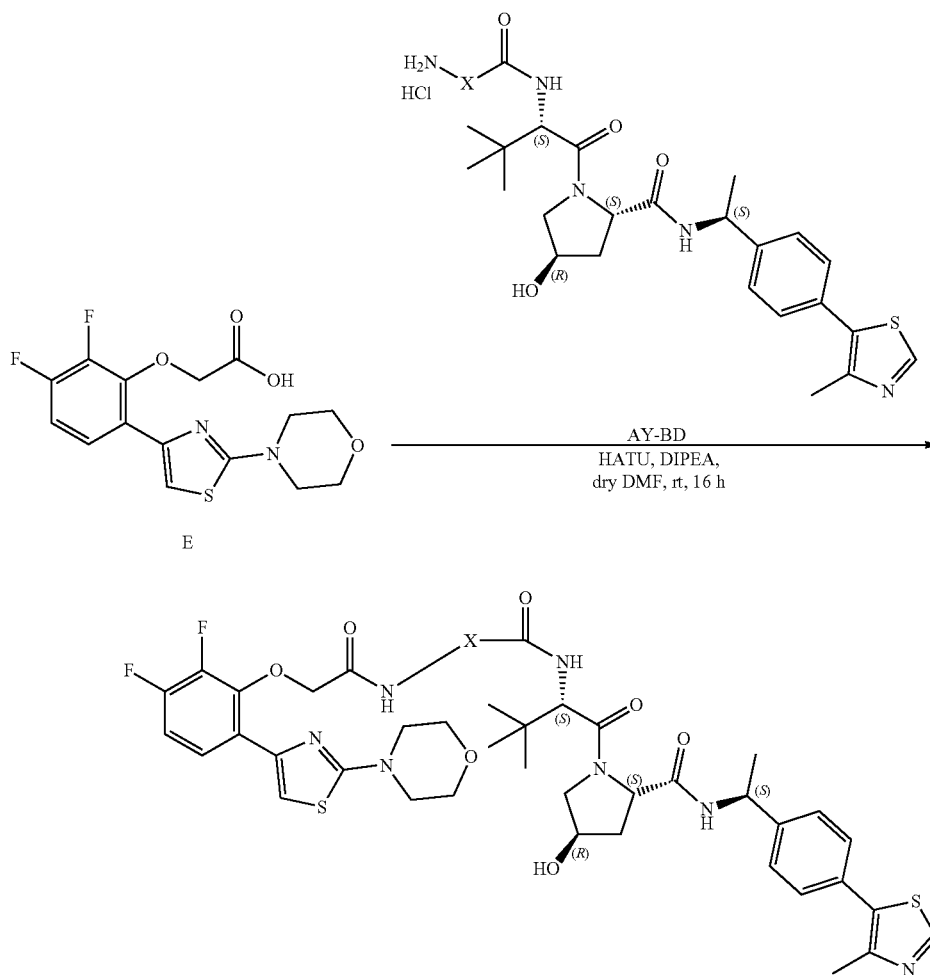
Scheme 8. Synthesis of Examples 15-20
