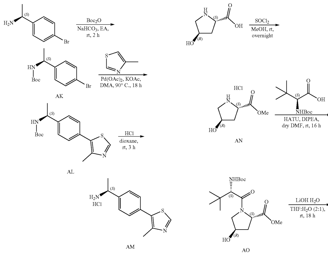
Scheme 7: Synthesis of VHL-based E3LB-3 moiety and linker connection
