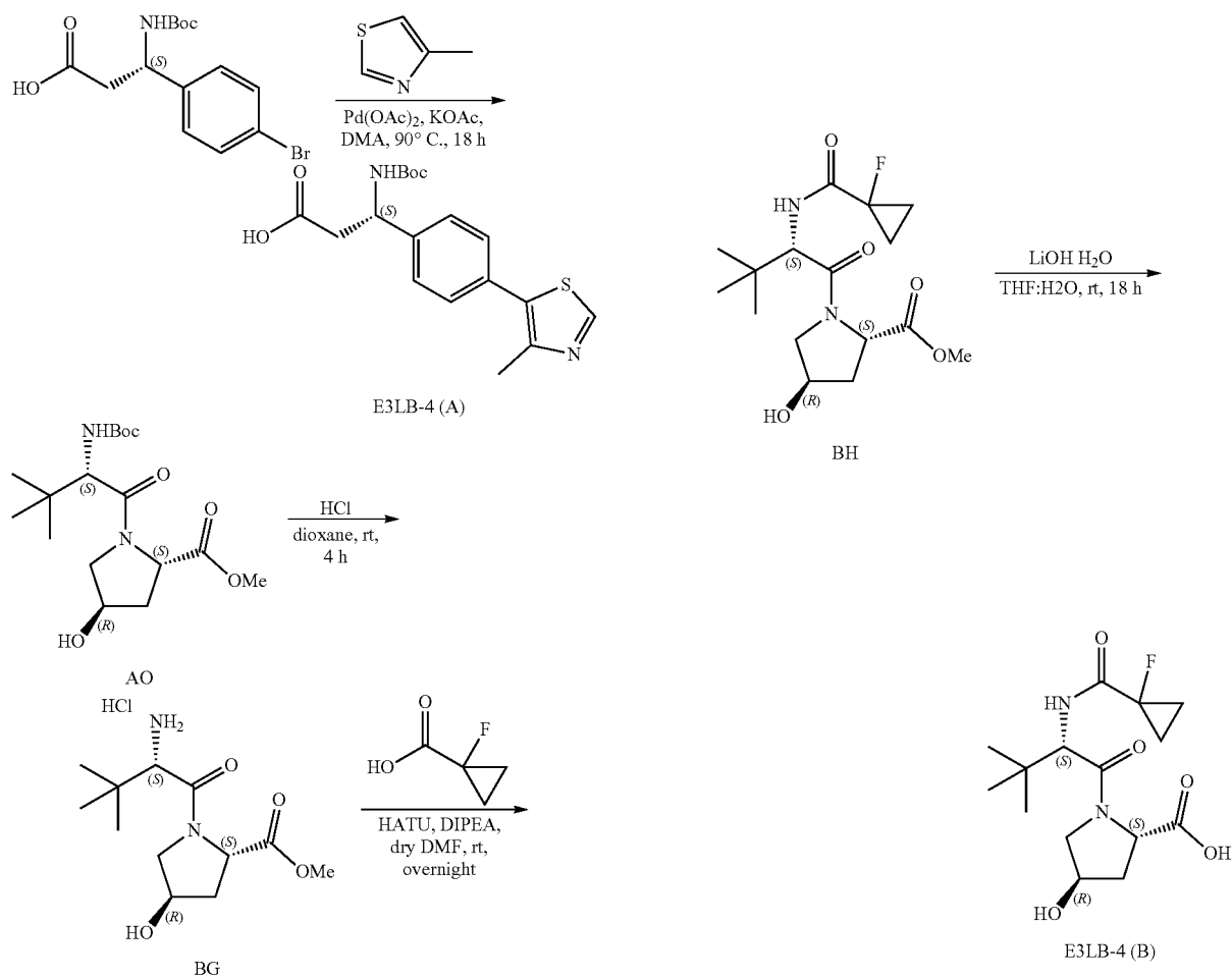
Scheme 10. Synthesis of VHL-based E3LB-4 moieties
