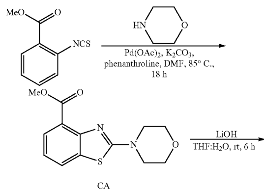
Scheme 15. Synthesis of ARB-2 moiety
