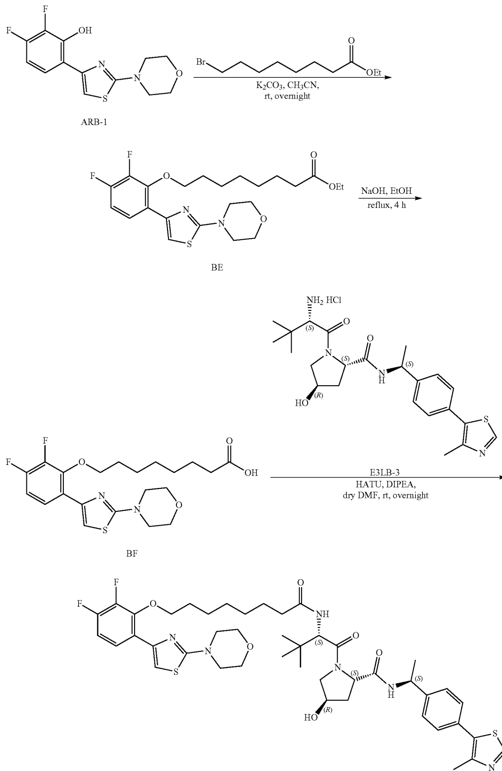
Scheme 9. Synthesis of Example 21
