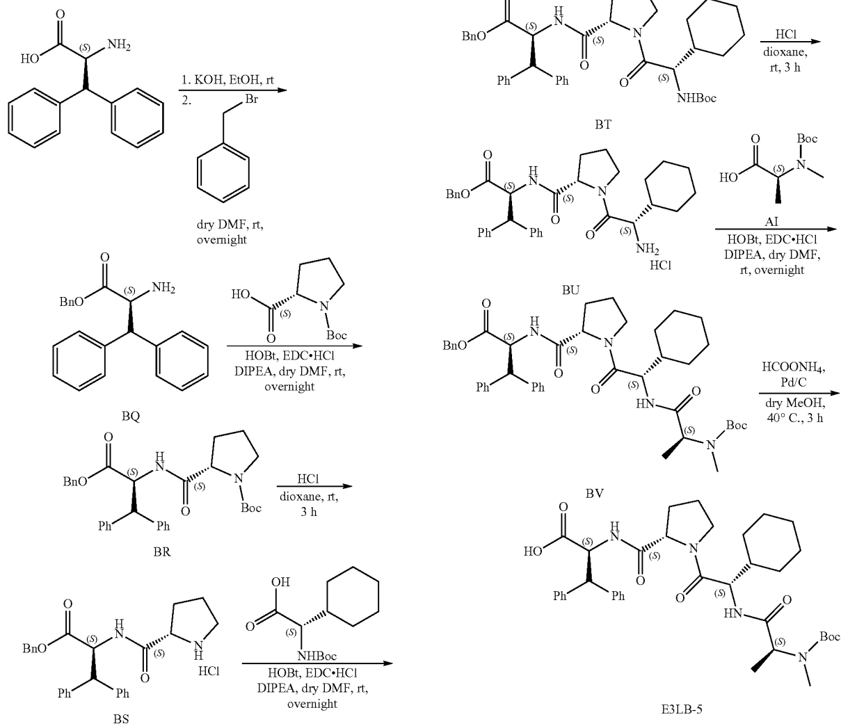
Scheme 12. Synthesis of IAP ligand-based E3LB-5 moiety
