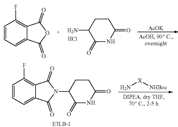
Scheme 2. Synthesis of pomalidomide-based E3LB-1 moiety and linker connection
