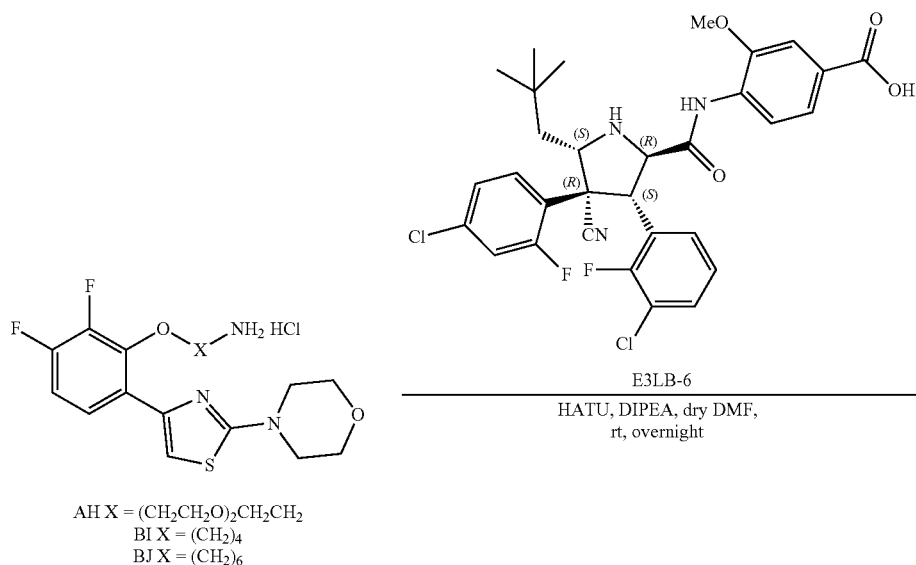
Scheme 14. Synthesis of Examples 27-29
