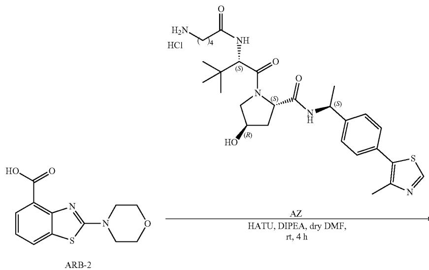
Scheme 16: Synthesis of Examples 30
