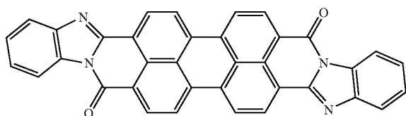
Pherylene compound
