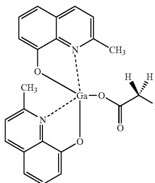
Gaq' 2 OAc
