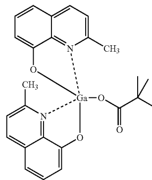
Gaq' 2 OPiv
