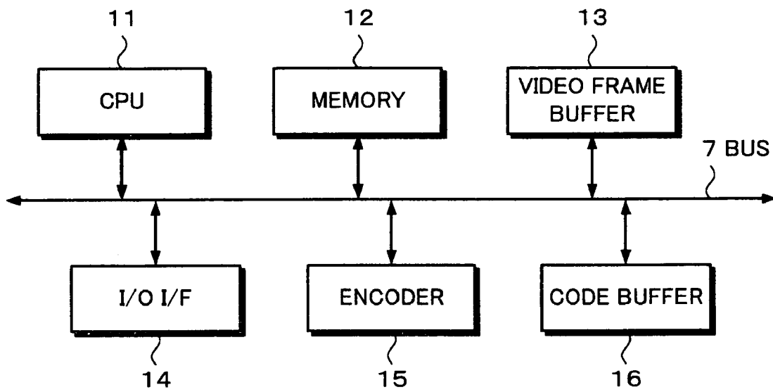
ENCODING APPARATUS 10
