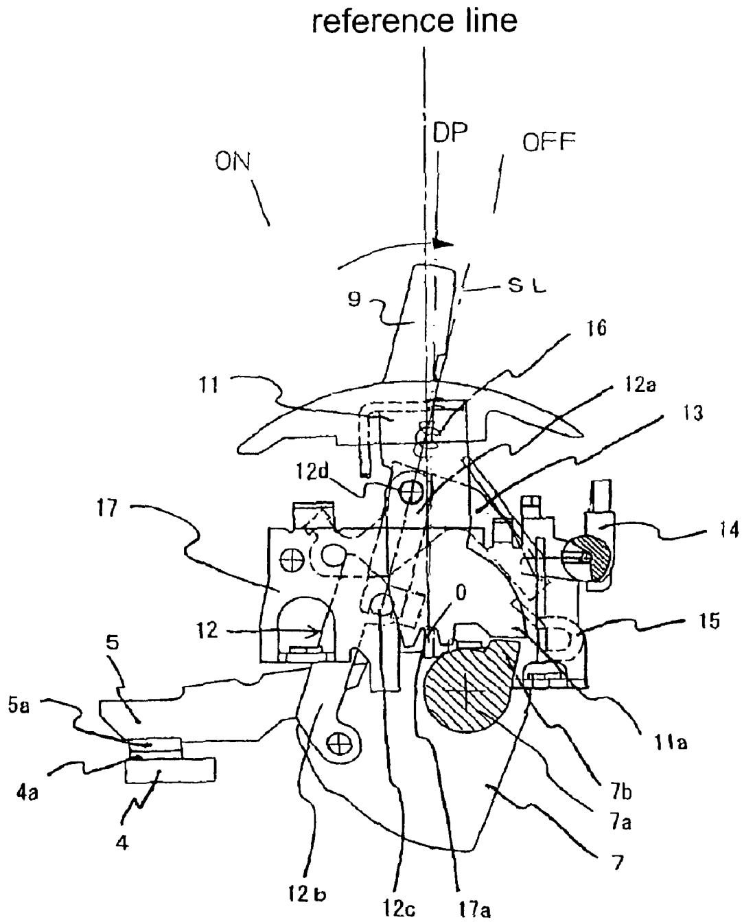
Fig. 7 Prior Art
