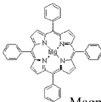
Magnesium Tetraphenyl Porphyrin
