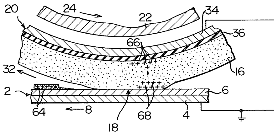
FIG. 3-B PRIOR ART
