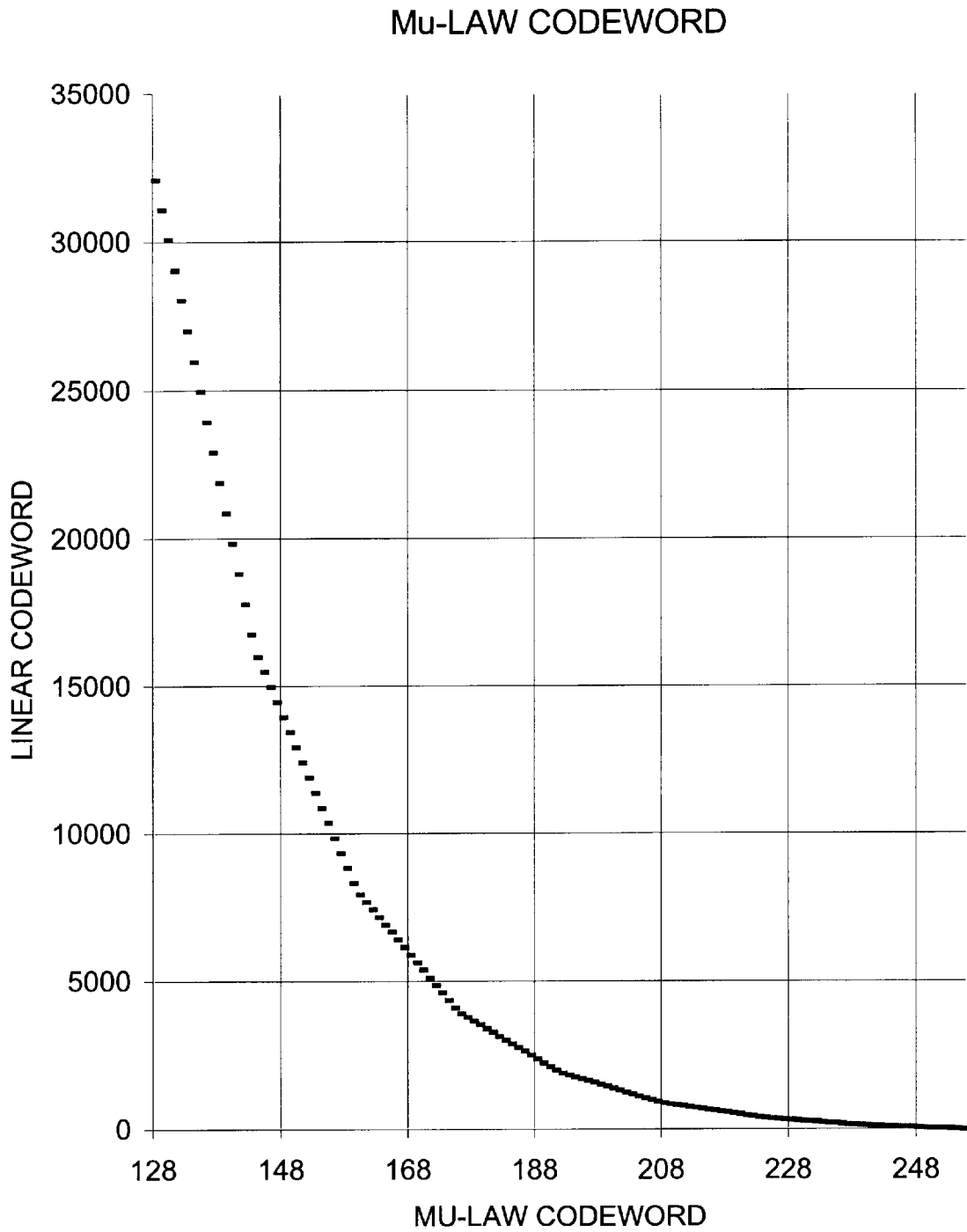
Fig. 3 Prior Art
