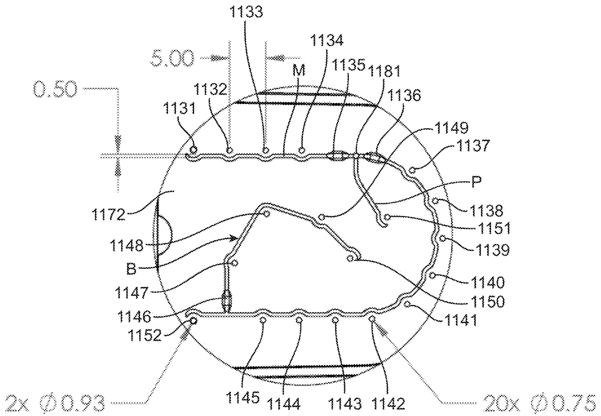
DETAIL C
