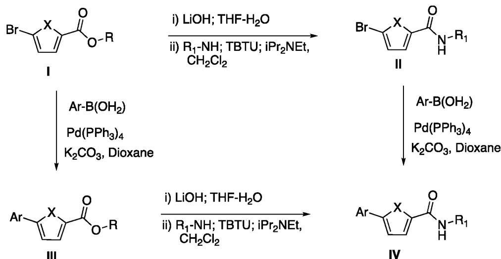
Scheme 1. General synthetic procedures for preparation of ERR analogs.
