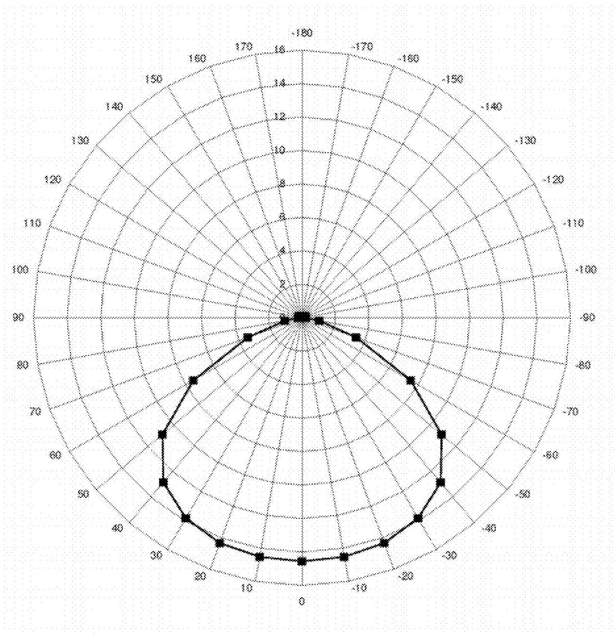
POLAR CANDELA DISTRIBUTION PLOT
