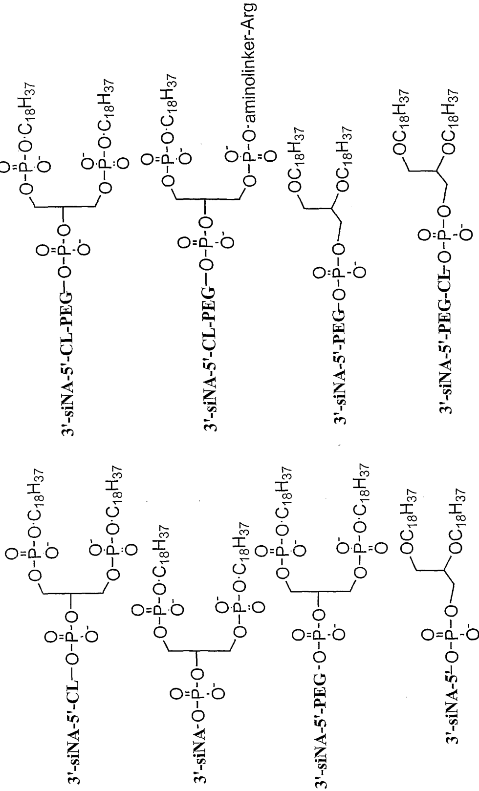
Figure 51: siNA/Phospholipid Conjugates
