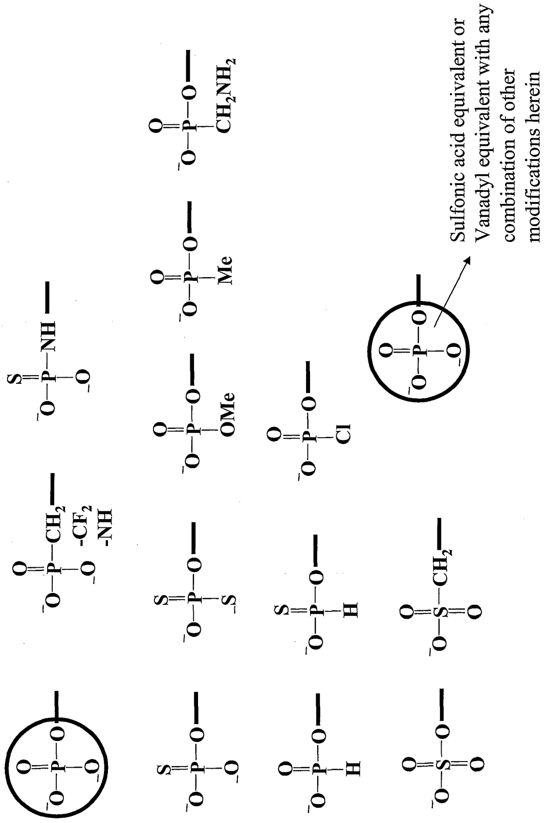
Figure 75: 5'-phosphate modifications
