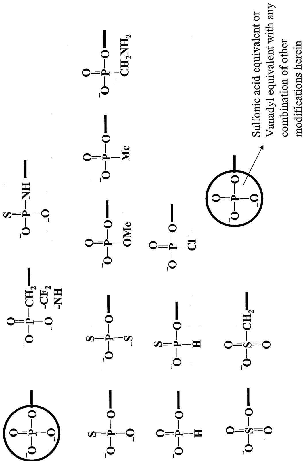
Figure 79: 5'-phosphate modifications
