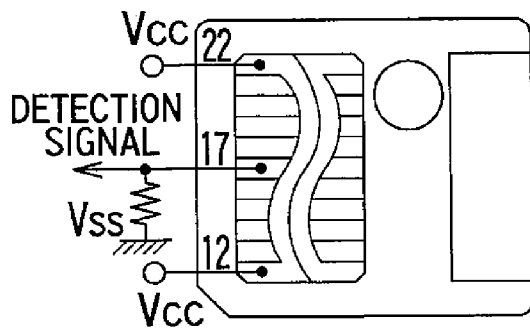
5V PRODUCT
