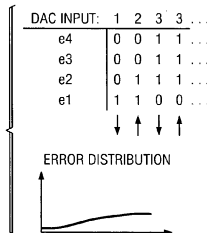
FIG. 4 (PRIOR ART)
