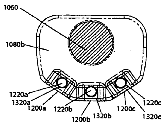
Fig. 12 (Section B-B of Fig. 7 )
