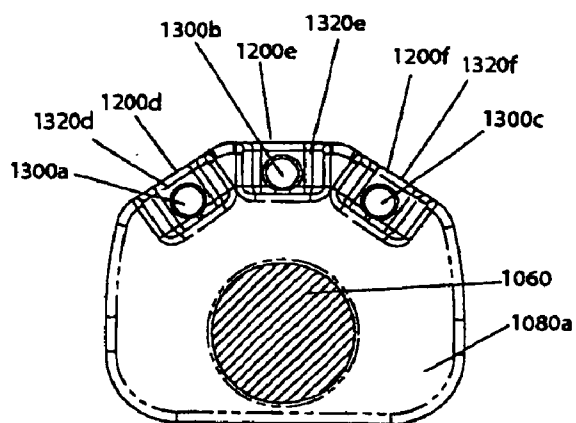
Fig. 11 (Section A-A of Fig. 7 )
