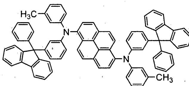
1,6mMemFLPAPrn
