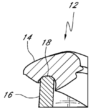
FIG. 3 (Prior Art)
