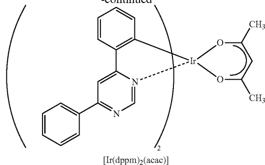
[Ir(dppm) 2 (acac)]
