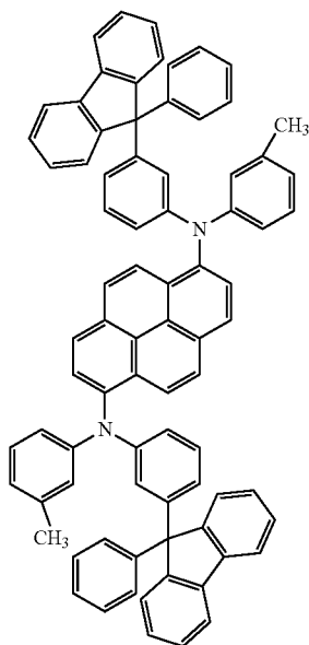
1,6MemFLPAPm
