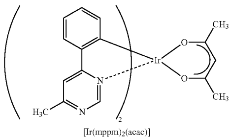
[Ir(mppm) 2 (acac)]
