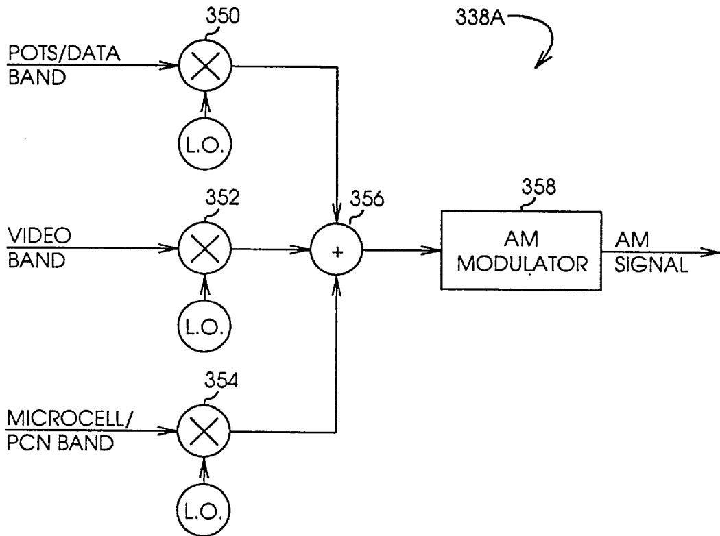
AM Modulator
