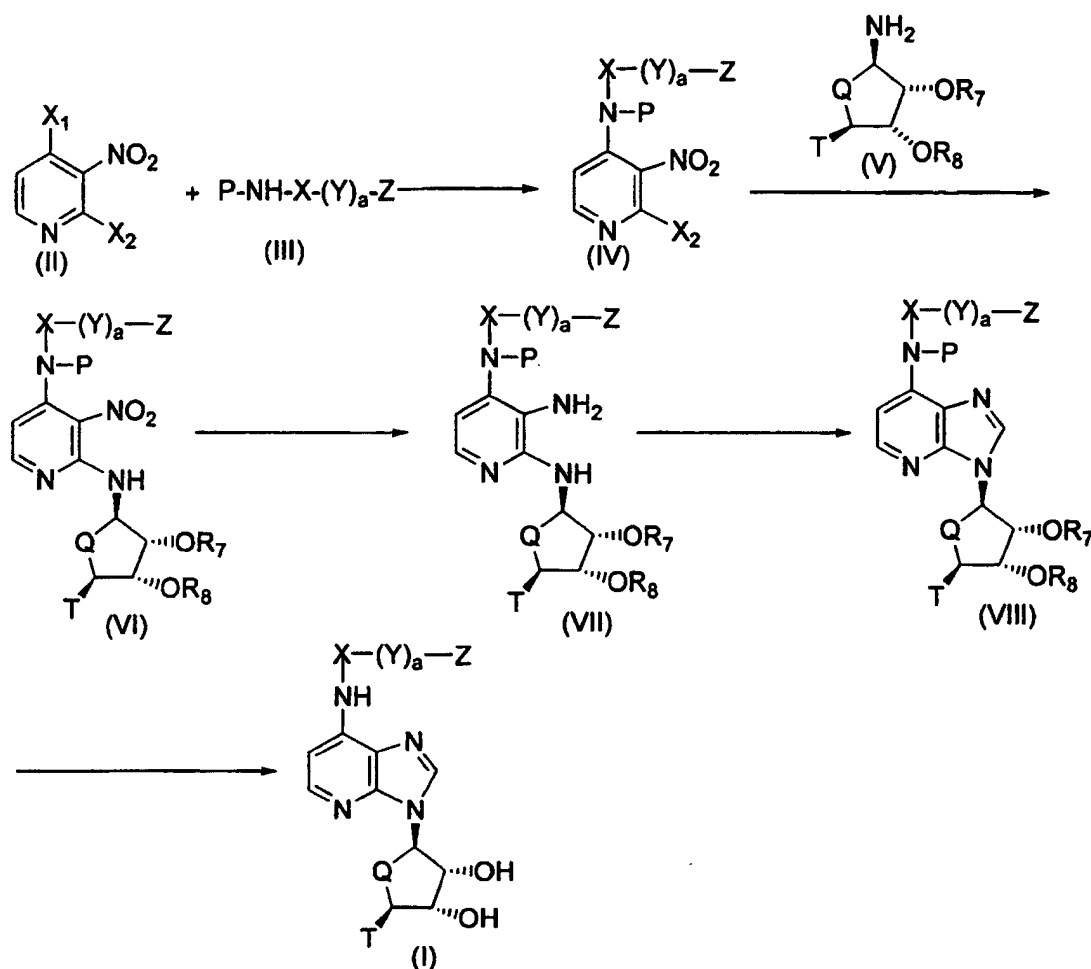
Scheme 1
