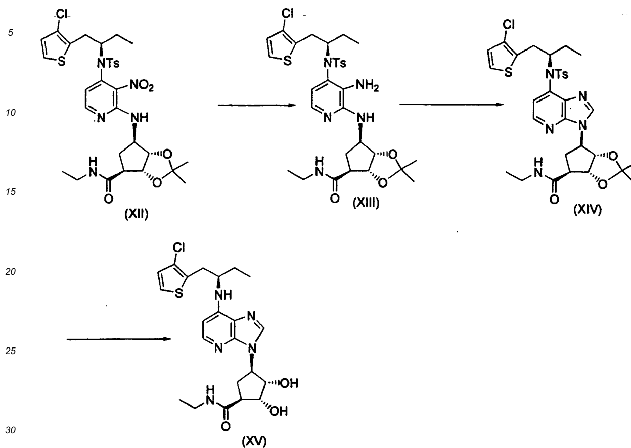
Scheme 2, con't.
