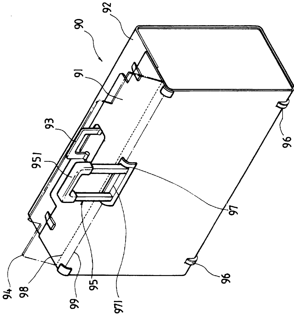
FIG 1 PRIOR ART
