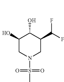
(3R, 4R, 5S)-5-(difluoromethyl)-1-(methylsulfonyl)piperidine-3,4-diol
