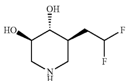
(3R, 4R, 5S)-5-(2,2-difluoroethyl) piperidine-3,4-diol
