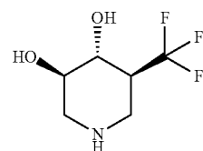
(3R, 4R, 5S)-5-(trifluoromethyl) piperidine-3,4-diol
