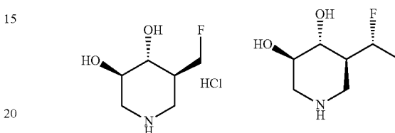
(3R, 4R, 5S)-5-(fluoromethyl) piperidine-3,4-diol hydrochloride
