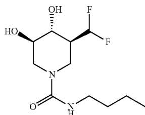
(3S, 4R, 5R)-N-butyl-3-(difluoromethyl)-4,5-dihydroxypiperidine-1-carboxamide
