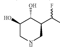
(3R, 4R, 5S)-5-(1-fluoroethyl)piperidine-3,4-diol
