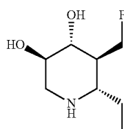
(3R, 4R, 5S, 6S)-6-ethyl-5-(fluoromethyl) piperidine-3,4-diol
