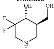
(4R, 5R)-3,3-difluoro-5-(hydroxymethyl) piperidin-4-ol
