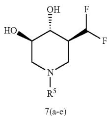
(3R,4R,5S)-1-Butyl-5-(difluoromethyl)piperidine 3,4-diol (General Procedure D) (7a; R 5 =Bu)
