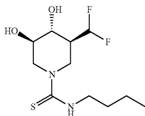
(3S, 4R, 5R)-N-butyl-3-(difluoromethyl)-4,5-dihydroxypiperidine-1-carbothioamide
