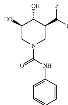
(3S, 4R, 5R)-3-(difluoromethyl)-4,5-dihydroxy-N-phenylpiperidine-1-carboxamide
