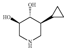
(3R, 4R, 5S)-5-cyclopropylpiperidine- 3,4-diol
