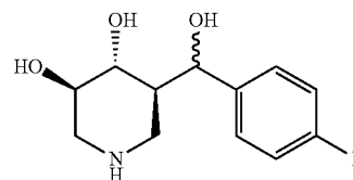
(3R, 4R, 5R)-5-(4-fluorophenyl)(hydroxymethyl)piperidine-3,4-diol
