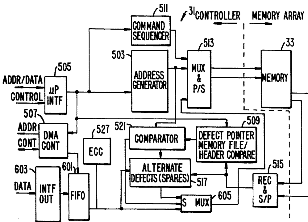
WRITE DATA PATH CONTROL
