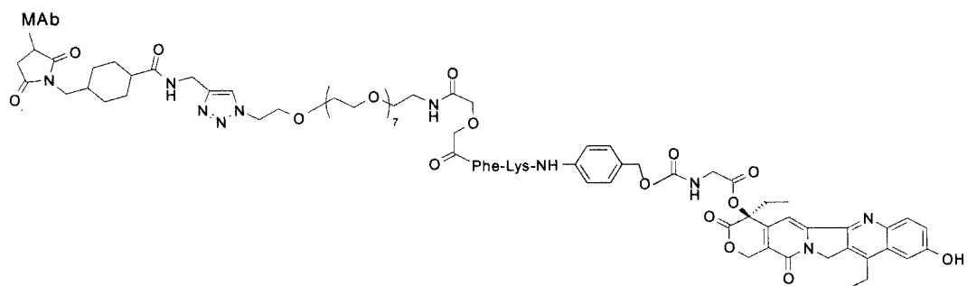
MAb-CL3-SN-38
