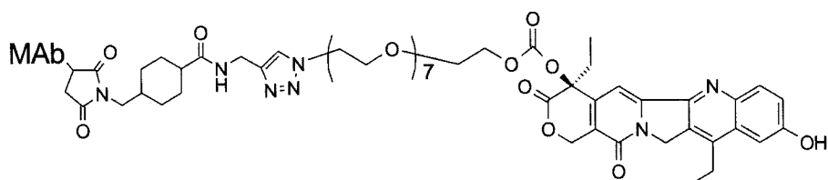
MAb-CL5-SN-38.
