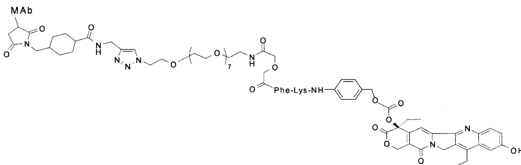
MAb-CL2-SN-38
