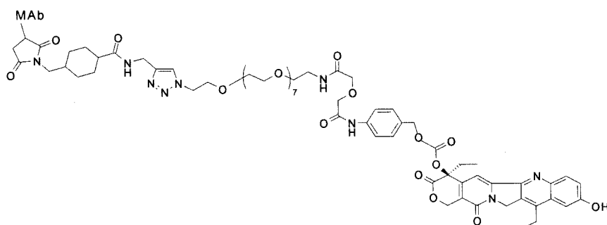
MAb-CL4-SN-38, or
