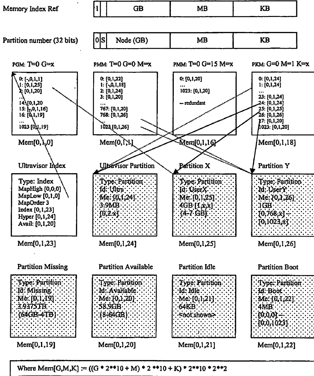
Figure 8 : Partition Memory Map
