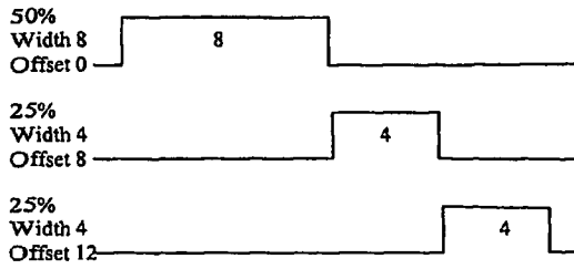
Figure 5 : Processor Sharing
