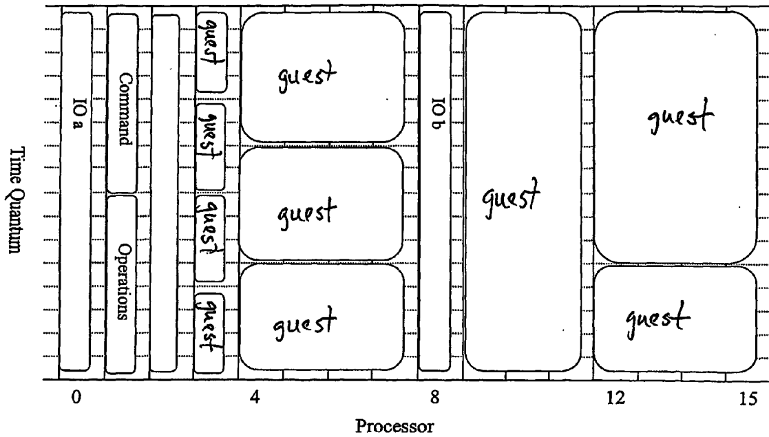
Figure 6 : Processor Schedule
