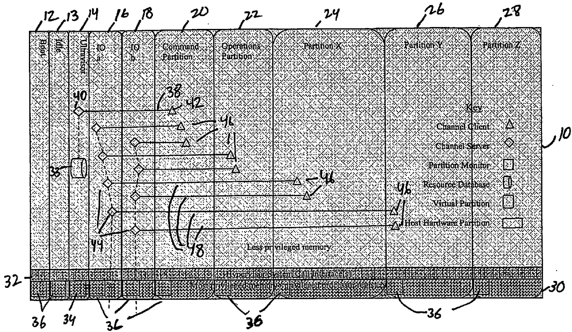
Figure 3: Partition Channels
