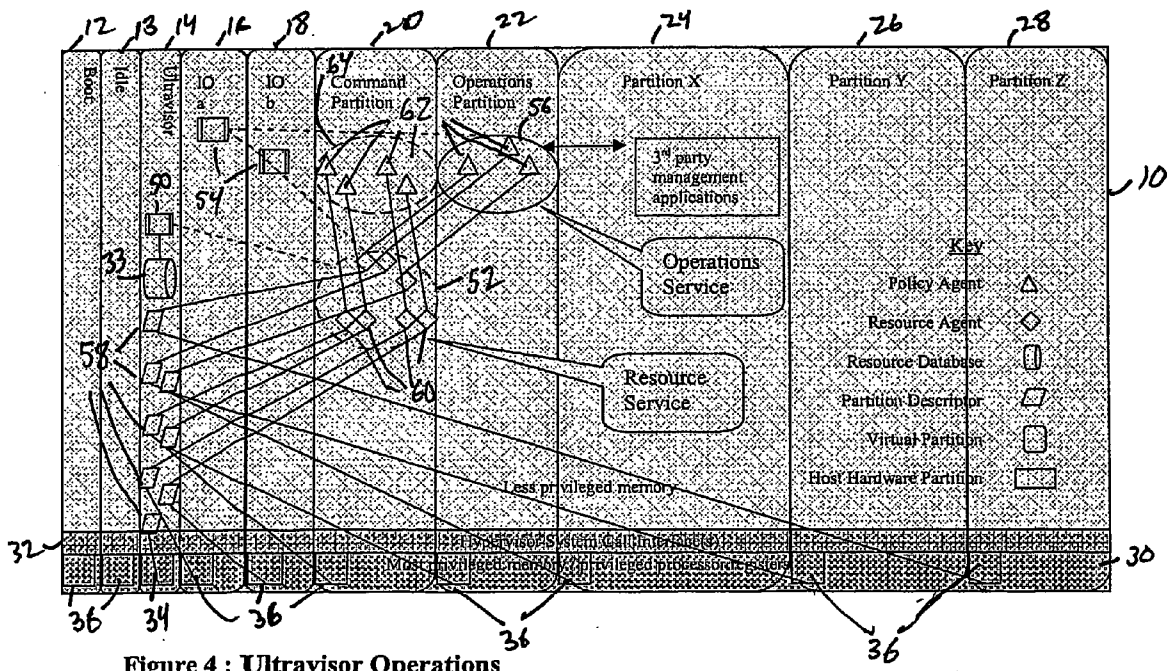
Figure 4: Ultravisor Operations
