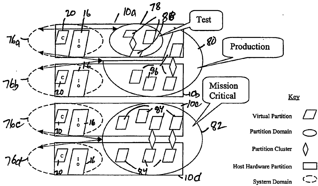
Figure 11 : Ultravisor Domains
