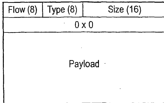
Example of a packet with a tag
