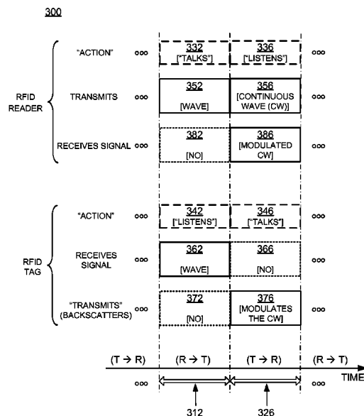
RFID SYSTEM COMMUNICATION
