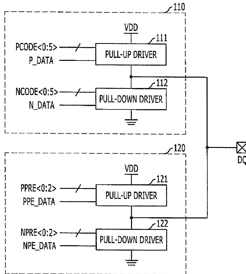
FIG. 1 (PRIOR ART)
