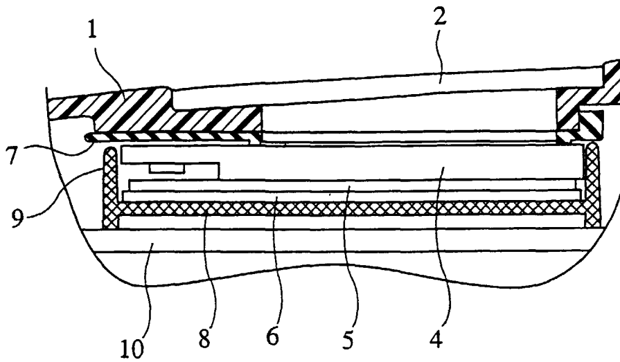
FIG.10 (PRIOR ART)
