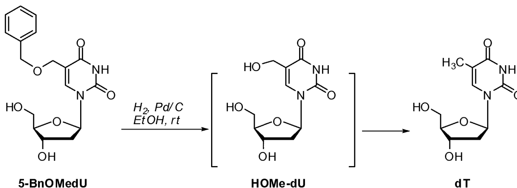
Scheme 42. Catalytic hydrogenolysis of 5-benzyloxymethyl-2'-deoxyuridine
