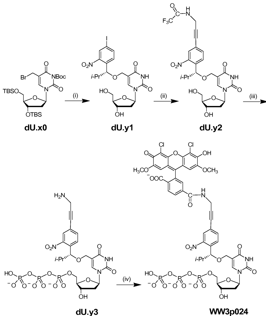
Scheme 14. Synthesis of 6-JOE labeled 5- \{(R) -1-[4-(3-amino-1-propynyl)-2-nitrophenyl]-2-methyl-propyloxy}methyl-2'-deoxyuridine-5'-triphosphate. (i) (R)-1-(4-iodo-2-nitrophenyl)-
