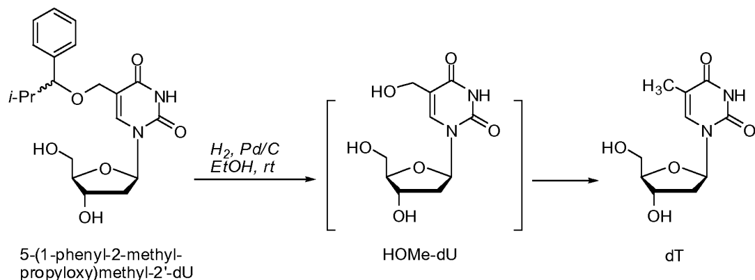
Scheme 43. Catalytic hydrogenolysis of 5-(1-phenyl-2-methyl-propyloxy)methyl-2'-deoxyuridine
