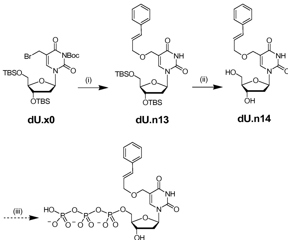
Scheme 37. Synthesis of 5-(3-phenyl-2-propenyloxy)methyl-2'-deoxyuridine-5'-triphosphate.
