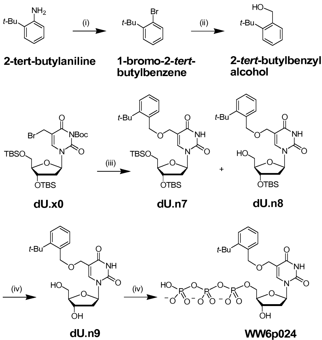
Scheme 34. Synthesis of 5-(2-tert-butylbenzyloxy)methyl-2'-deoxyuridine-5'-triphosphate.
