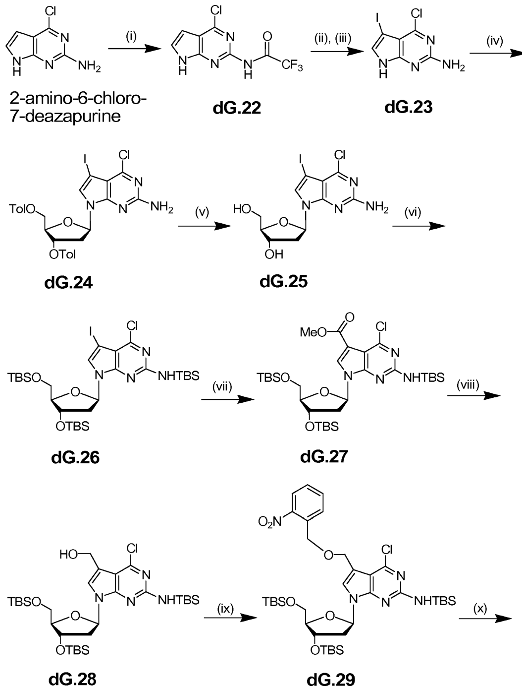
5 Scheme 19. Synthesis of 7-(2-nitrobenzyloxy)methyl-7-deaza-2'-deoxyguanosine-5'-triphosphate. (i) TFAA, pyridine (anh.), room temperature, 91% (ii) NIS, CH 2 Cl 2 (anh.),
